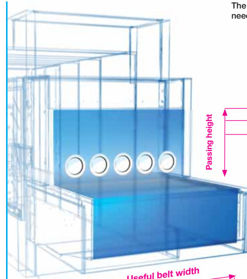
Whether basket or conveyor transport, the M-iQ fits perfectly with a selection of conveyor dimensions and useful belt widths.
