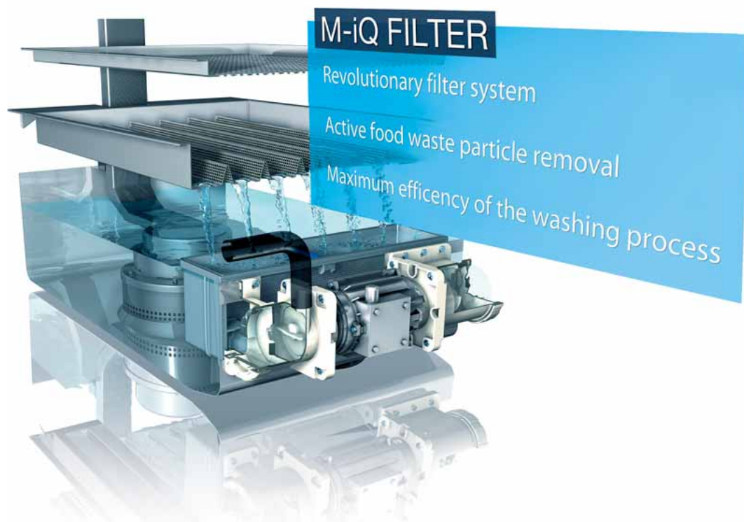
Triple-layered system: coarse filter, fine filter and M-iQ filter unit
